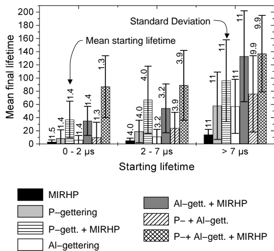
Figure 3: Mean final lifetime values after different processing steps (see Fig. 1) calculated for regions of different starting lifetimes.
