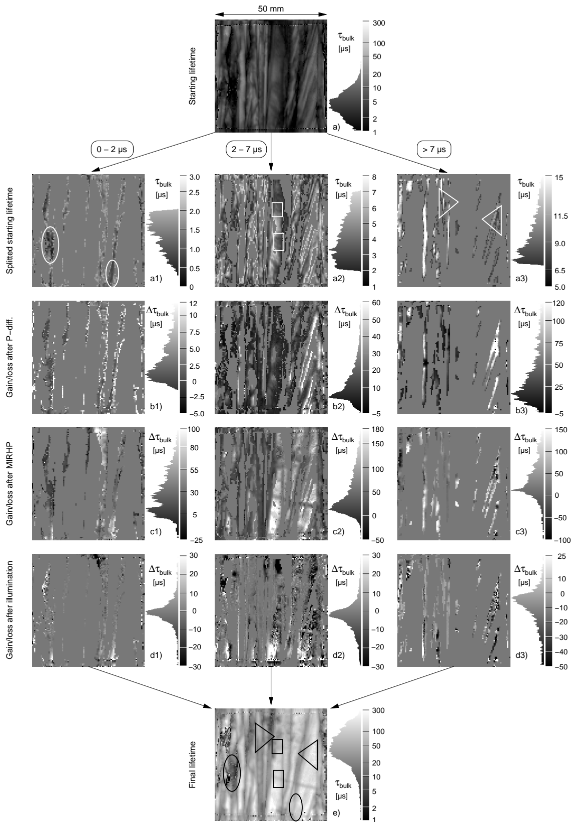
Figure 2: Bulk lifetime mappings of wafer 2 as obtained after appropriate combination of various measurements that lead to reliable high and low lifetime values. Mappings have been split according to their starting lifetimes. Graphs (a), (ax) and (e) show absolute lifetime values, whereas (bx), (cx) and (dx) illustrate gains or losses caused by each processing step as related to the lifetime values measured before this individual step.
