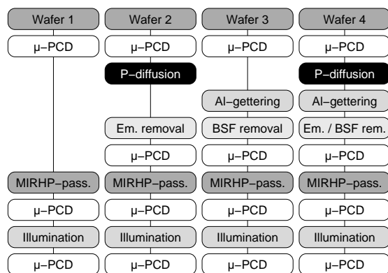
Figure 1: Structure of the experiment. After various successive processing steps spatially resolved bulk lifetime measurements have been performed.
