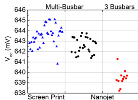
Figure 3: Open circuit voltages of the 3 groups. Advantage in voltage for group 1 can be seen because of dual printing.
