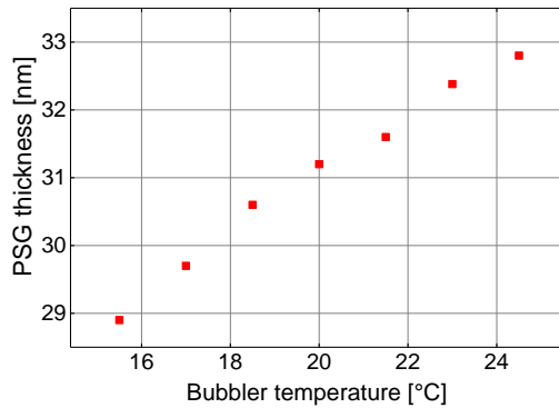
Figure 2: PSG thickness in dependence of bubbler temperature, measured with spectroscopic ellipsometry.
