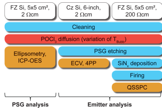
Figure 1: Sample preparation for PSG and emitter characterization. For POCl 3 diffusion, several bubbler temperatures (T Bubb ) were used.
