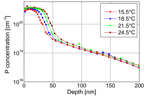
Figure 4: Emitter profiles in dependence of bubbler temperature, measured with ECV. The measurement was performed in the center of the wafer.
