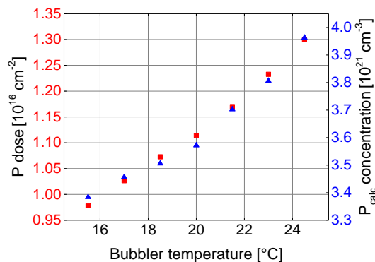
Figure 3: P dose in the PSG (left y-axis), measured with ICP-OES and calculated lower limit for P concentration in the PSG (right y-axis) as a function of \text{POCl}_3 bubbler temperature.
