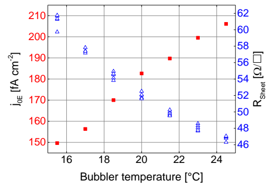
Figure 5: The emitter saturation current density (left y-axis) in dependence on the bubbler temperature, measured with QSSPC at an injection density of 1.5 \cdot 10^{16} \text{ cm}^{-3} . The sheet resistance (right y-axis), is measured with 4PP for different bubbler temperatures.
