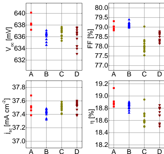
Figure 6: IV measurement: Emitter A is our reference with \text{POCl}_3\text{-N}_2 gas flow of \Phi_0 and bubbler temperature of 20^{\circ}\text{C} . Emitter B has a similar sheet resistance, by increasing \text{POCl}_3\text{-N}_2 gas flow and reducing bubbler temperature at the same time. For emitter C \text{POCl}_3\text{-N}_2 gas flow is reduced, while for emitter D bubbler temperature is reduced.
