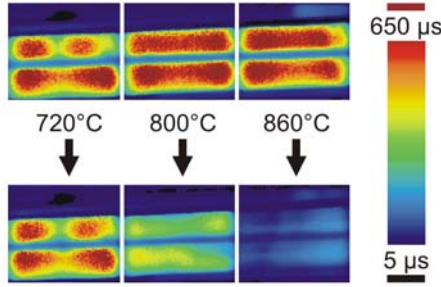
Figure 8: Detail of \mu\text{PCD} -measurements of adjacent EFG-Si-wafers, passivated by 30 nm \text{Al}_2\text{O}_3 and an additional 75 nm PECVD- \text{SiN}_x :H. The upper part shows the lifetime before, the lower part after a firing step at different peak temperatures.
