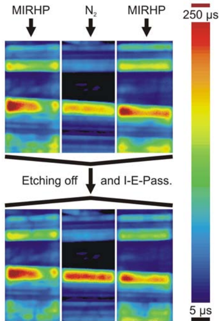
Figure 5: \mu PCD-measurements of EFG-Si, 5 nm Al 2 O 3 on both sides. The same three samples are shown with Al 2 O 3 passivation (top) and after etching off the Al 2 O 3 layer and a homogeneous chemical surface passivation by iodine-ethanol (I-E-Pass.) showing improved bulk passivation of the two samples with prior MIRHP treatment (bottom).
