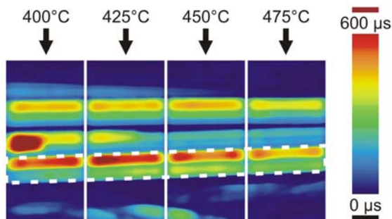
Figure 2: \mu PCD-measurements of EFG lifetime samples. The grains of interest proceed over four samples. The samples are passivated by 30 nm Al 2 O 3 and annealed at different temperatures between 400°C and 475°C.
