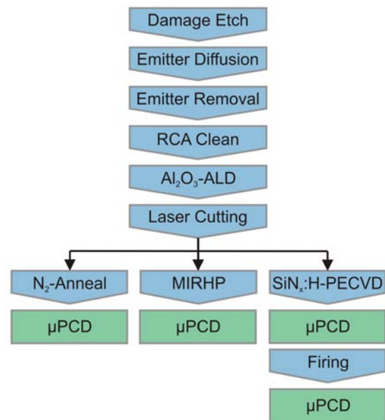
Figure 1: Processing sequence of p-doped 3 \Omega cm EFG lifetime samples. Passivation is performed by Al 2 O 3 , either annealed in N 2 ambience (left branch), after a MIRHP treatment (middle branch), or alternatively with PECVD-SiN x :H on top of the Al 2 O 3 layer (right branch).
