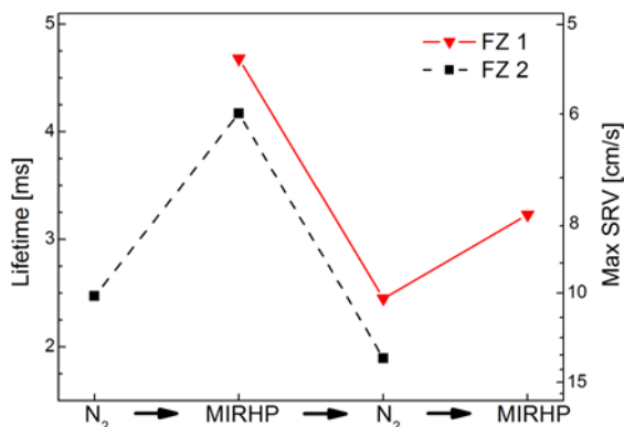
Figure 6: Transient-PCD-measurements of two 2 \Omega cm FZ samples, 5 nm Al 2 O 3 on both sides. The same samples are shown after annealing steps, alternately in N 2 atmosphere and MIRHP. A significant increase in minority carrier lifetime in consequence of exposure to atomic hydrogen can be seen (experiment comparable to the one shown in Figure 4).
