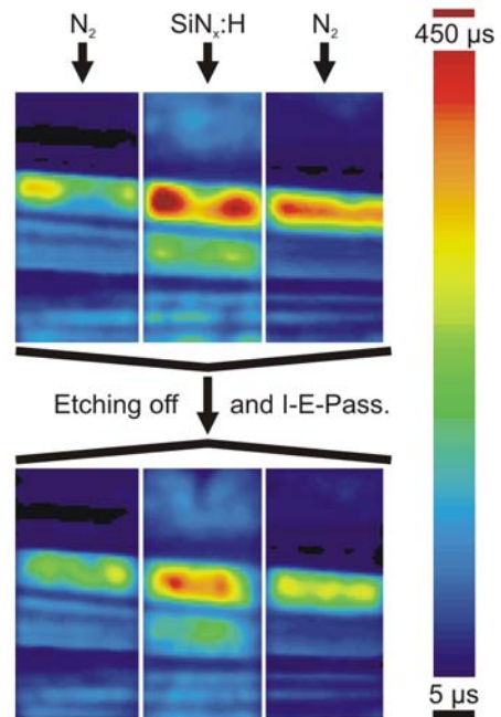
Figure 7: \mu PCD-measurements of three adjacent EFG wafers with the same grain structure, passivated by 7.5 nm Al 2 O 3 . The sample in the middle features an additional protection layer of 75 nm Si x :H. The higher lifetime values of this sample are also seen after etching off the dielectric passivation layers and a homogeneous chemical surface passivation (I-E-Pass.) suggesting a hydrogen passivation of the bulk during the PECVD of Si x :H.
