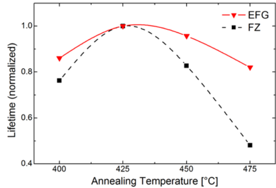
Figure 3: Lifetime values of samples passivated by 30 nm Al 2 O 3 and annealed at different temperatures. The optimum annealing temperature appears to be around 425°C.
