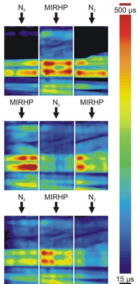
Figure 4: \mu PCD-measurements of EFG-Si, 5 nm Al 2 O 3 on both sides. The same three samples are shown after subsequent annealing steps, alternately in N 2 atmosphere and MIRHP. A significant increase in minority carrier lifetime in consequence of the hydrogen passivation is observable.
